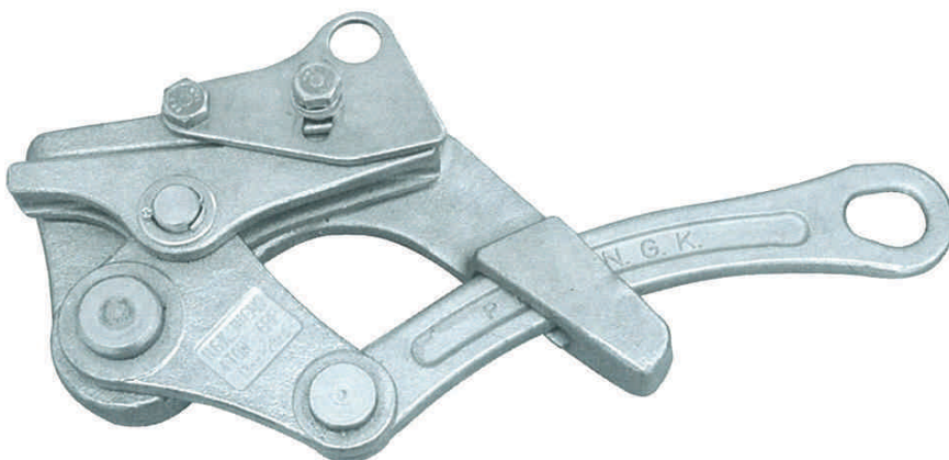
4t GRIP WITH SAFETY LATCH • 13 to 28mm (SMALL EYE) • 20 to 35mm (LARGE EYE)
